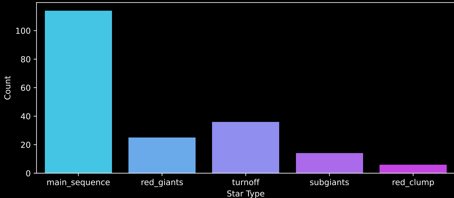
APOGEE DR17 Field: [160+61_MGA] Count plot of Star Type
