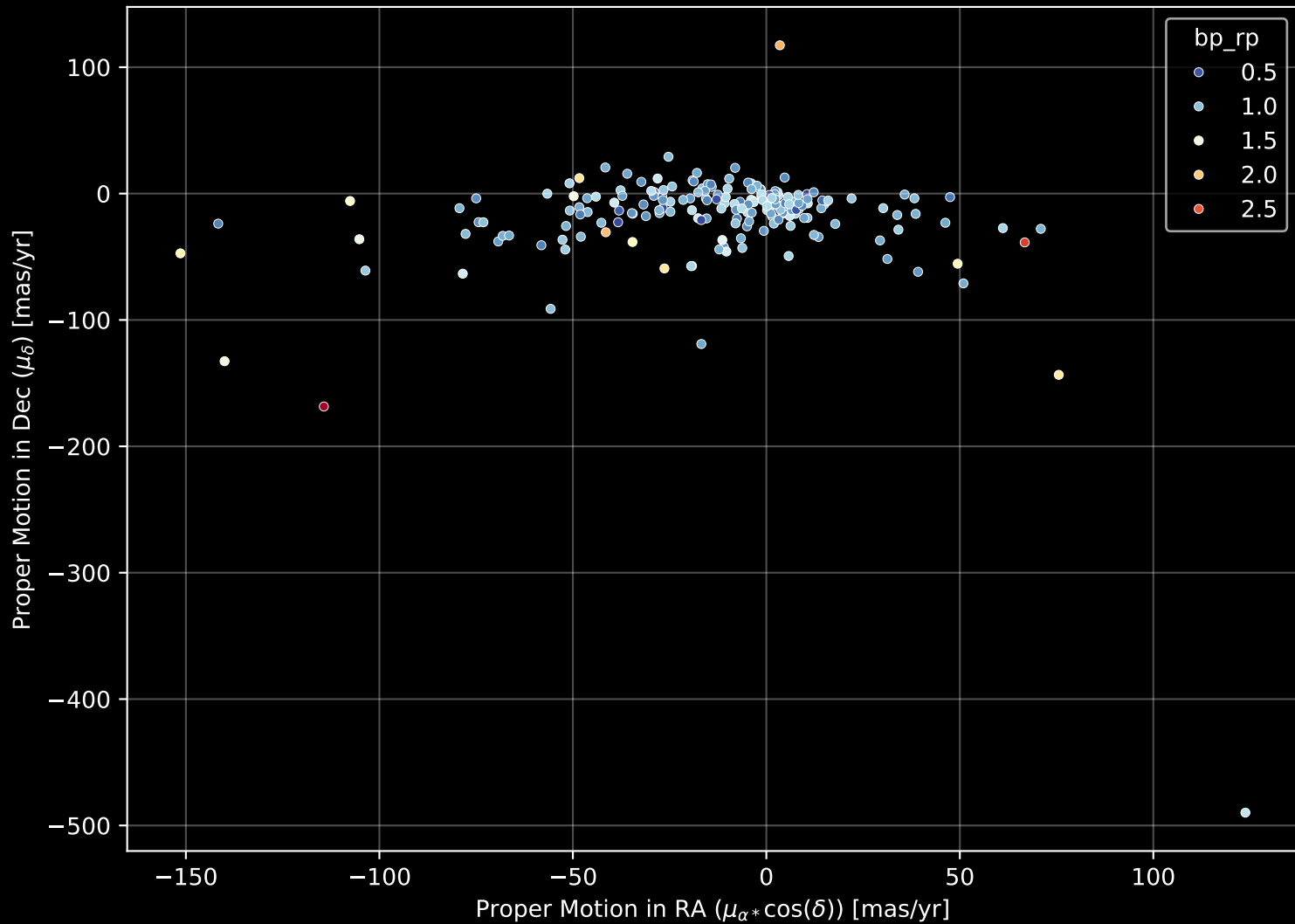
APOGEE DR17 Field: [160+61_MGA] Proper Motion Diagram (n= 195)
