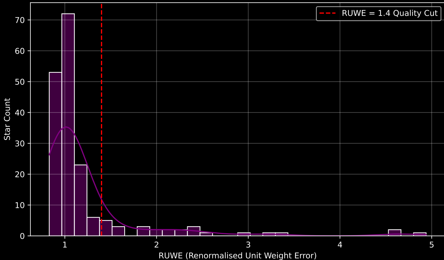
GAPOGEE DR17 Field [160+61_MGA] RUWE Distribution (n= 181)
