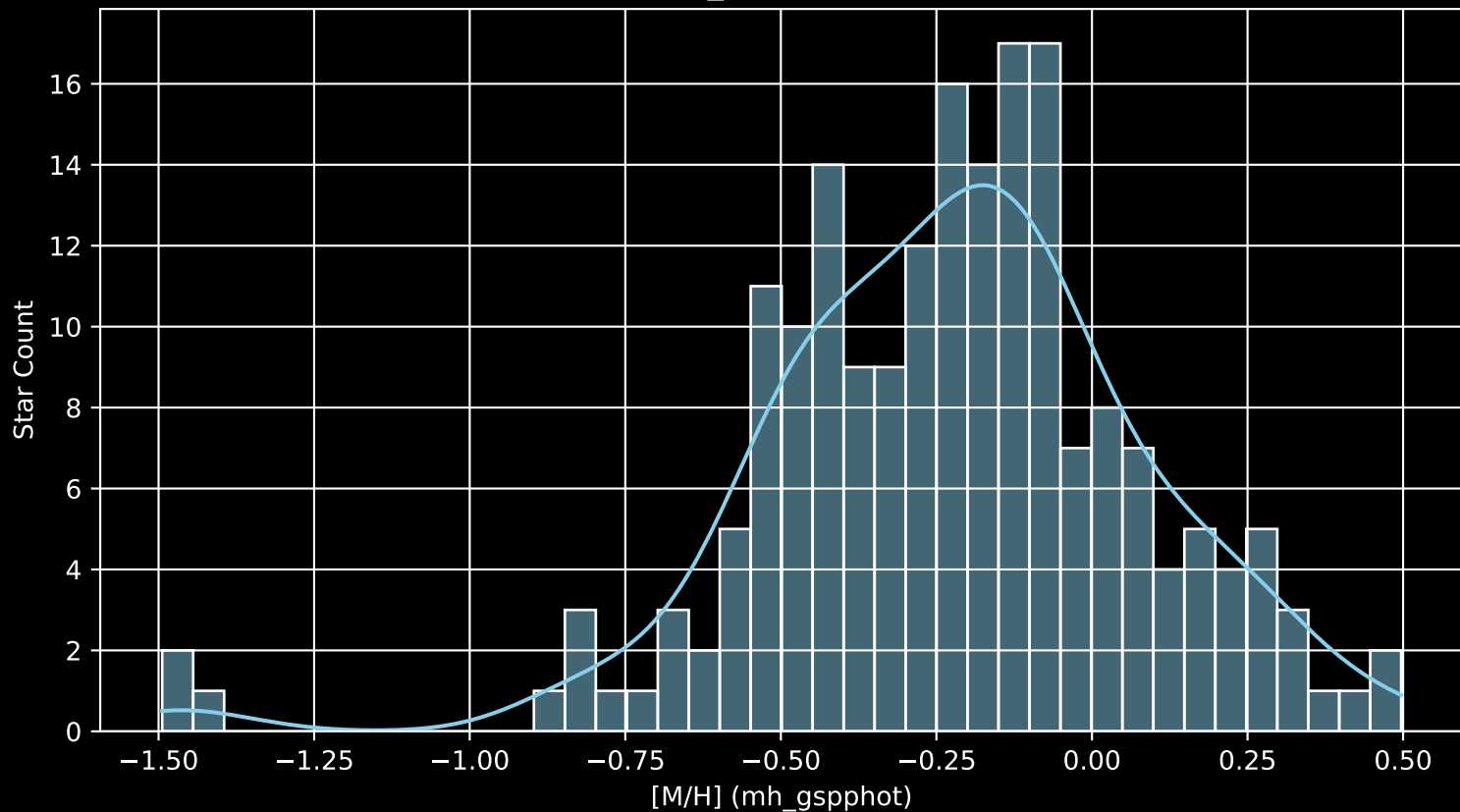
APOGEE DR17 Field: [160+61_MGA [M/H] (mh_gspphot) (n= 195)
