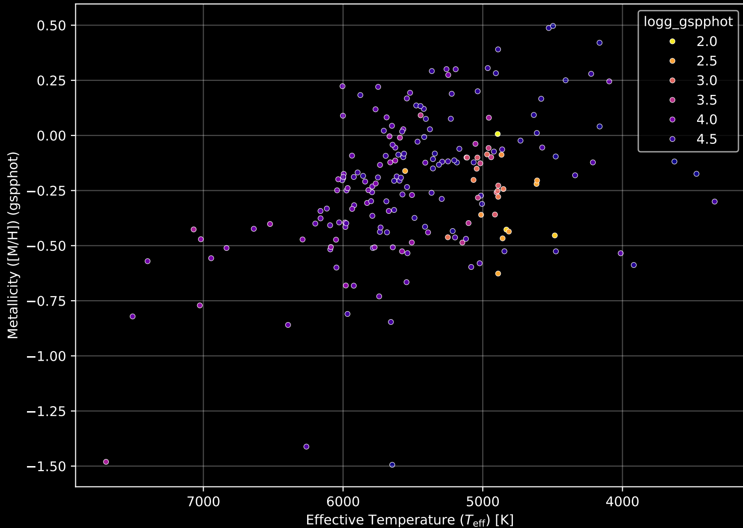
APOGEE DR17 Field: [160+61_MGA] Stellar Population Parameters (n= 195)
