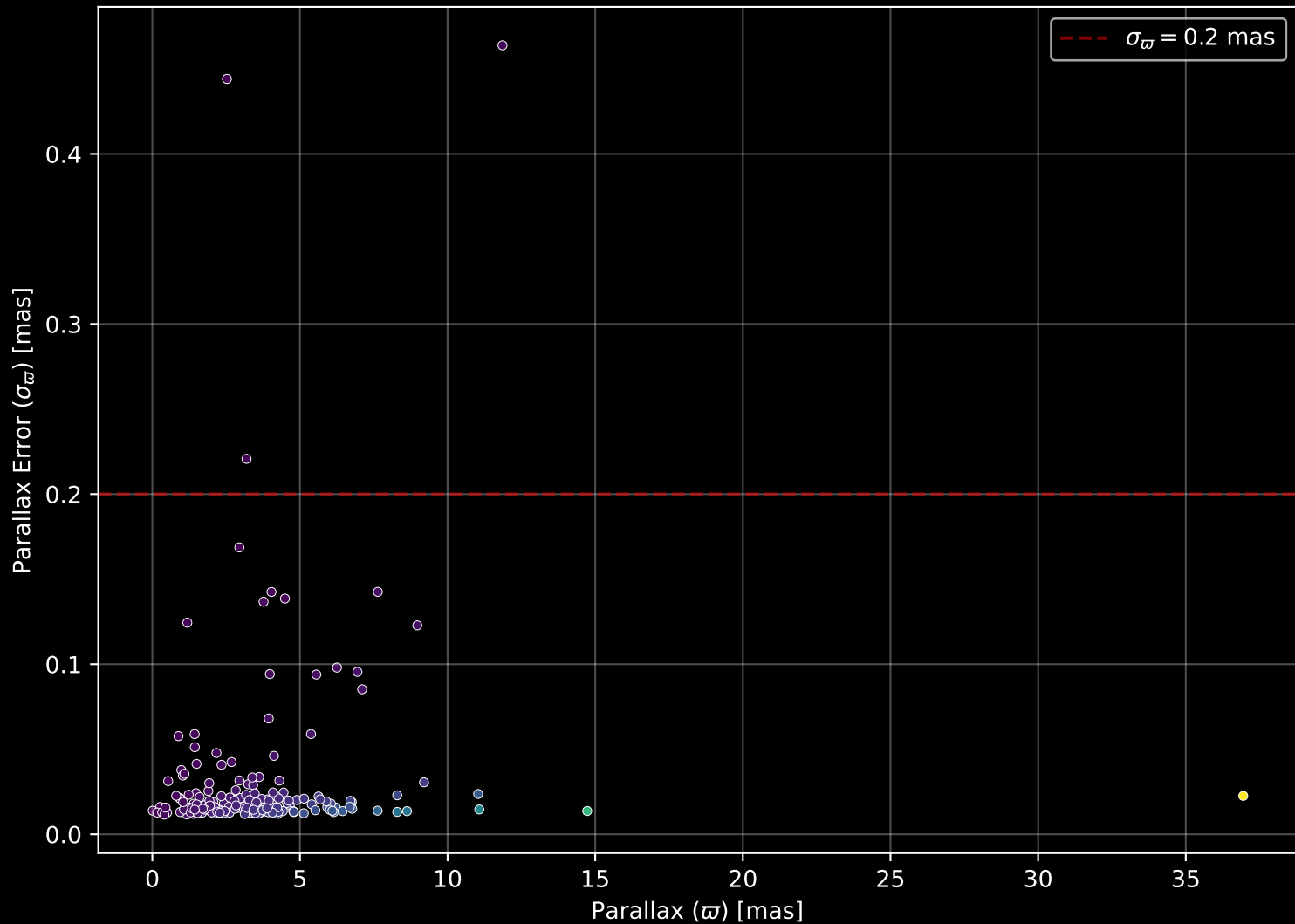
APOGEE DR17 Field: [160+61_MGA] Parallax Quality (n= 195)
